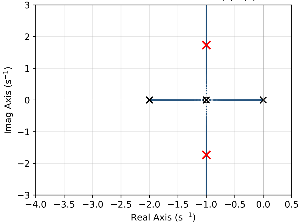
Problem 26: Root locus of D(s)G(s)
